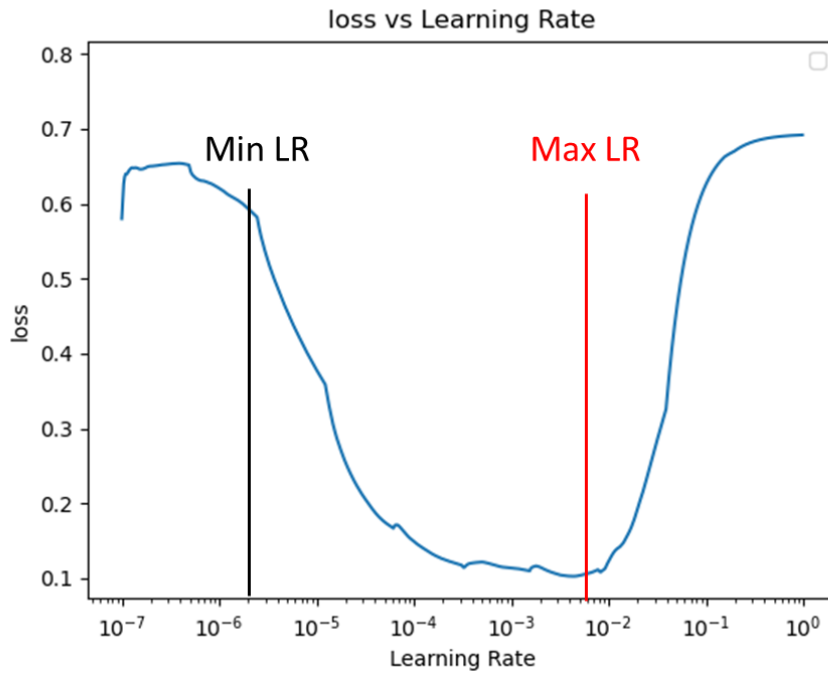
Supplementary Figure 1: Learning rate finder figure. The learning rate is gradually increased from 10e-7 to 10e-0 ; the point where loss begins to decrease is the minimum learning rate (min LR), and the point where it begins to increase is the maximum learning rate (max LR).
