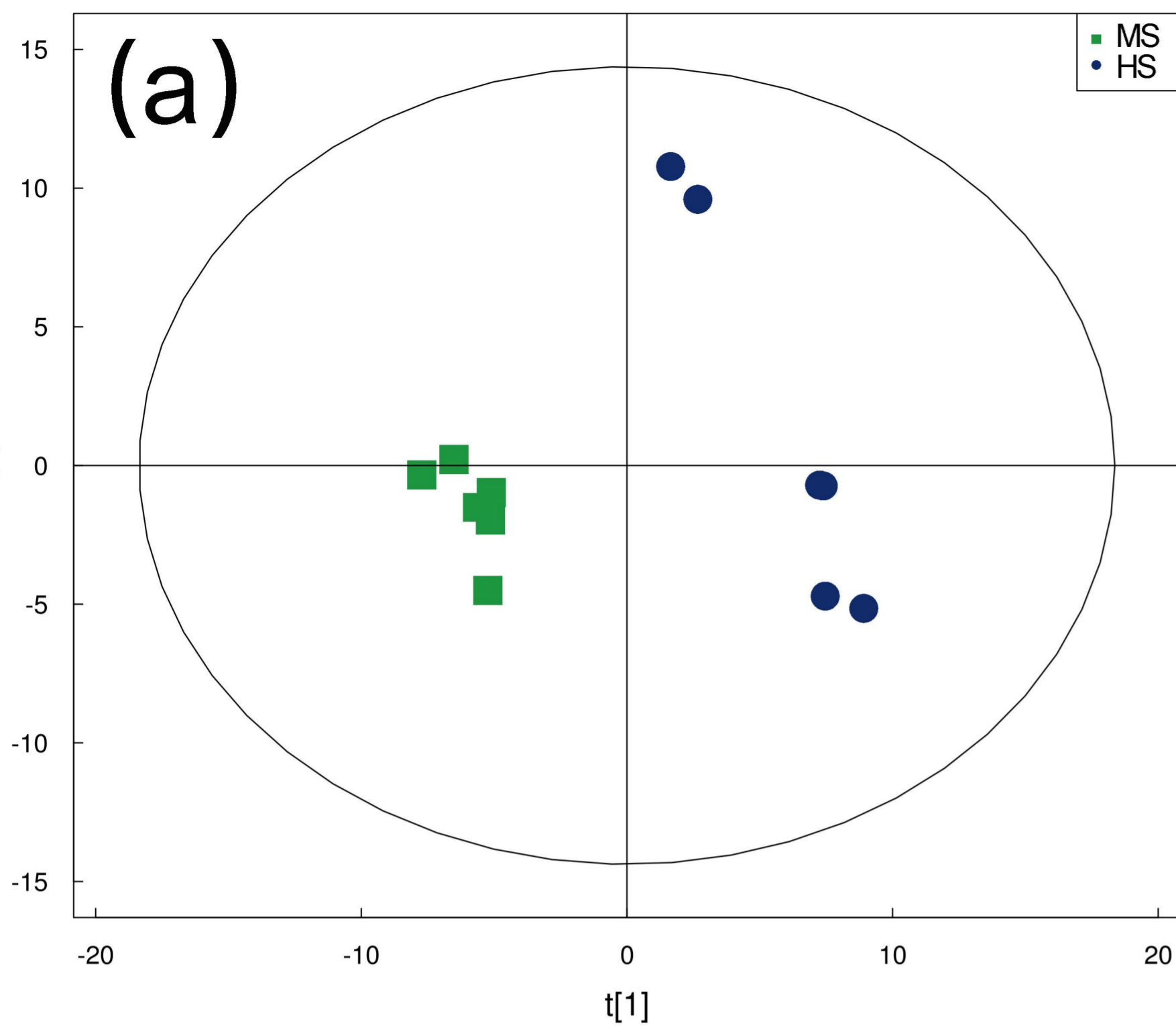
Scores (PLS-DA)
