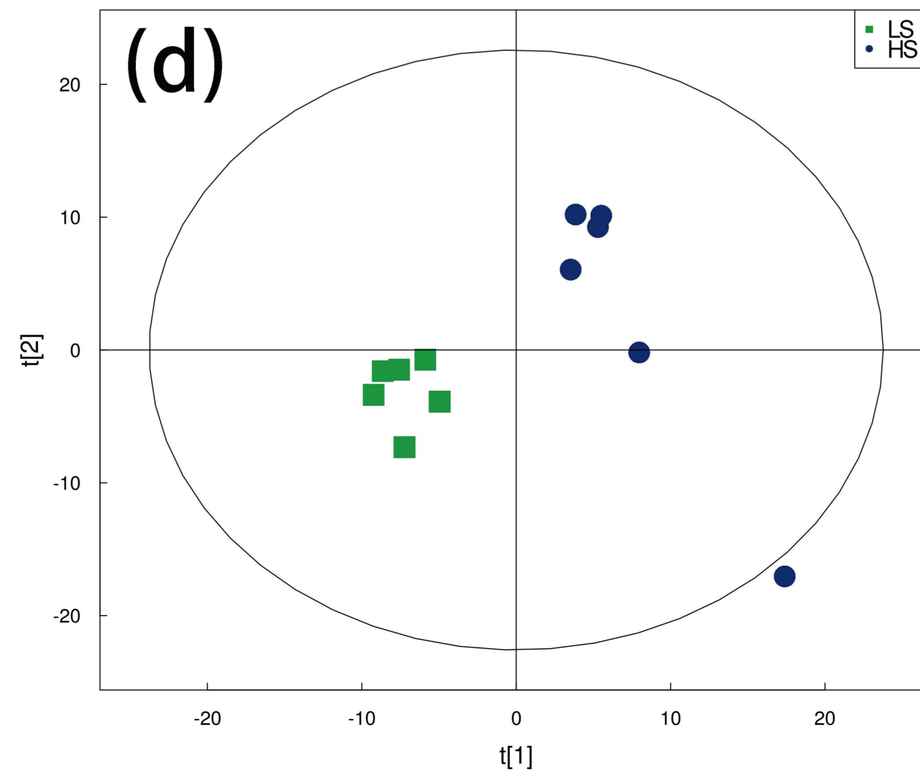
Scores (PLS-DA)
