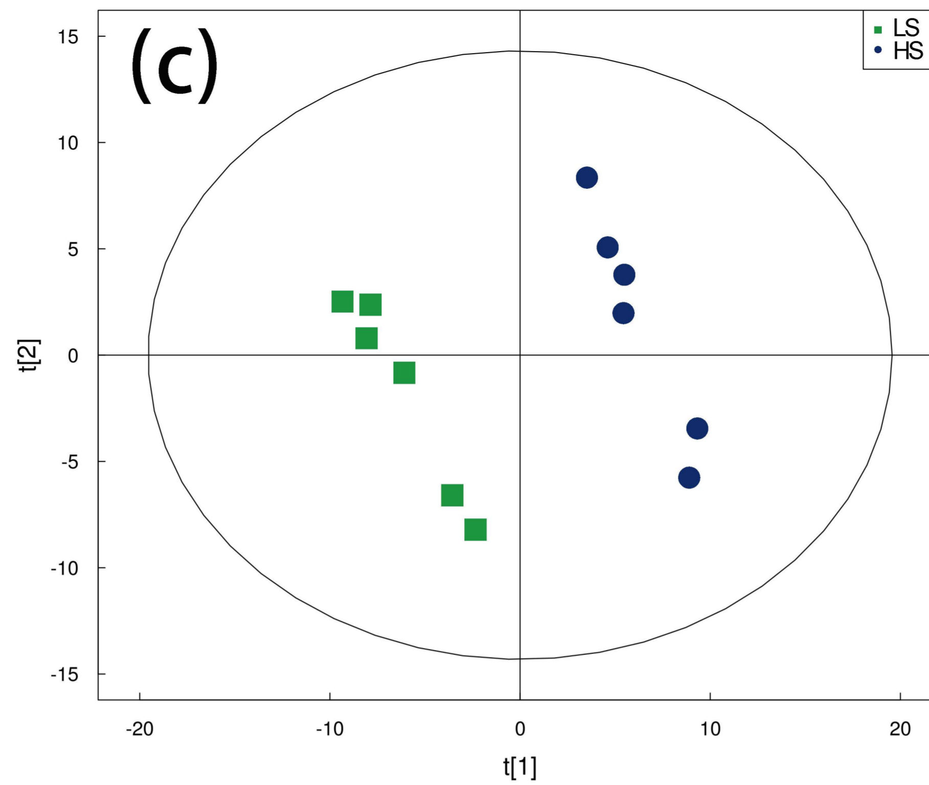
Scores (PLS-DA)
