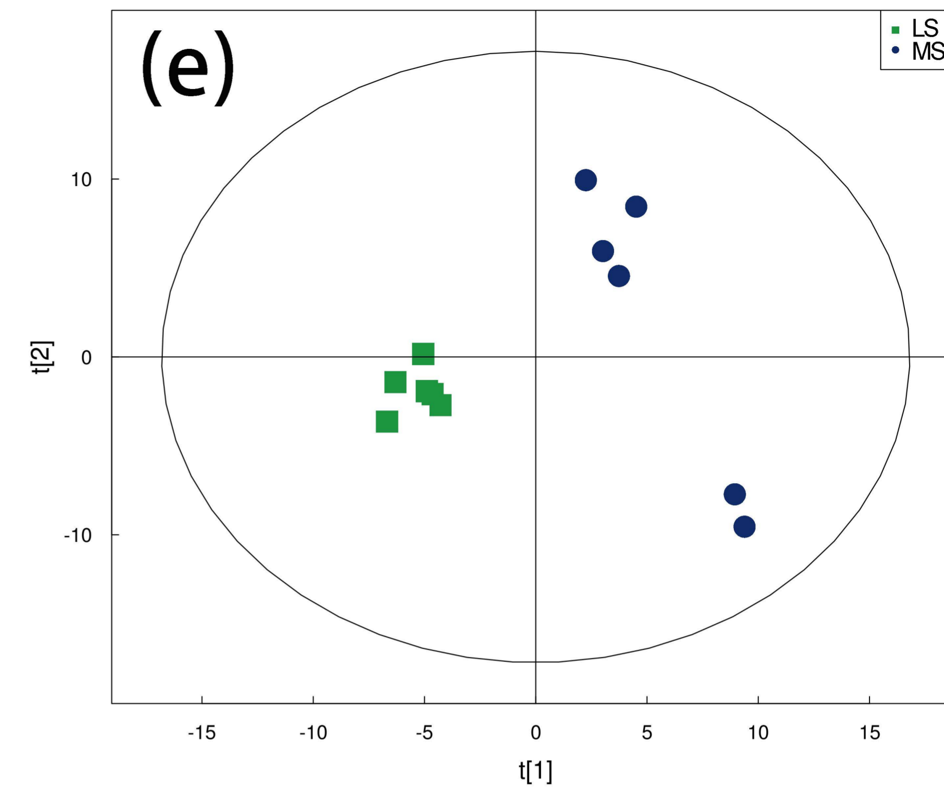
Scores (PLS-DA)
