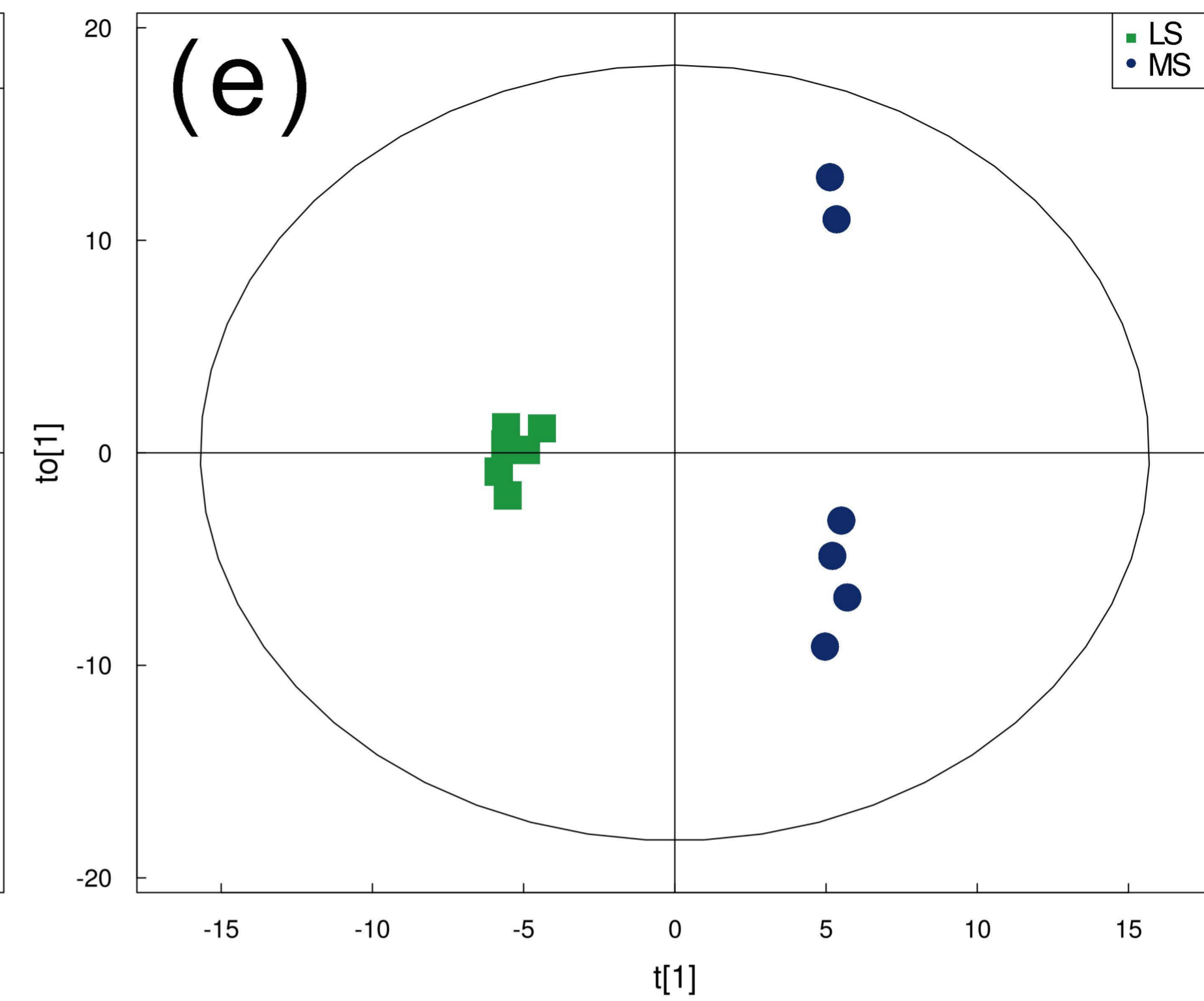
Scores (OPLS-DA)
