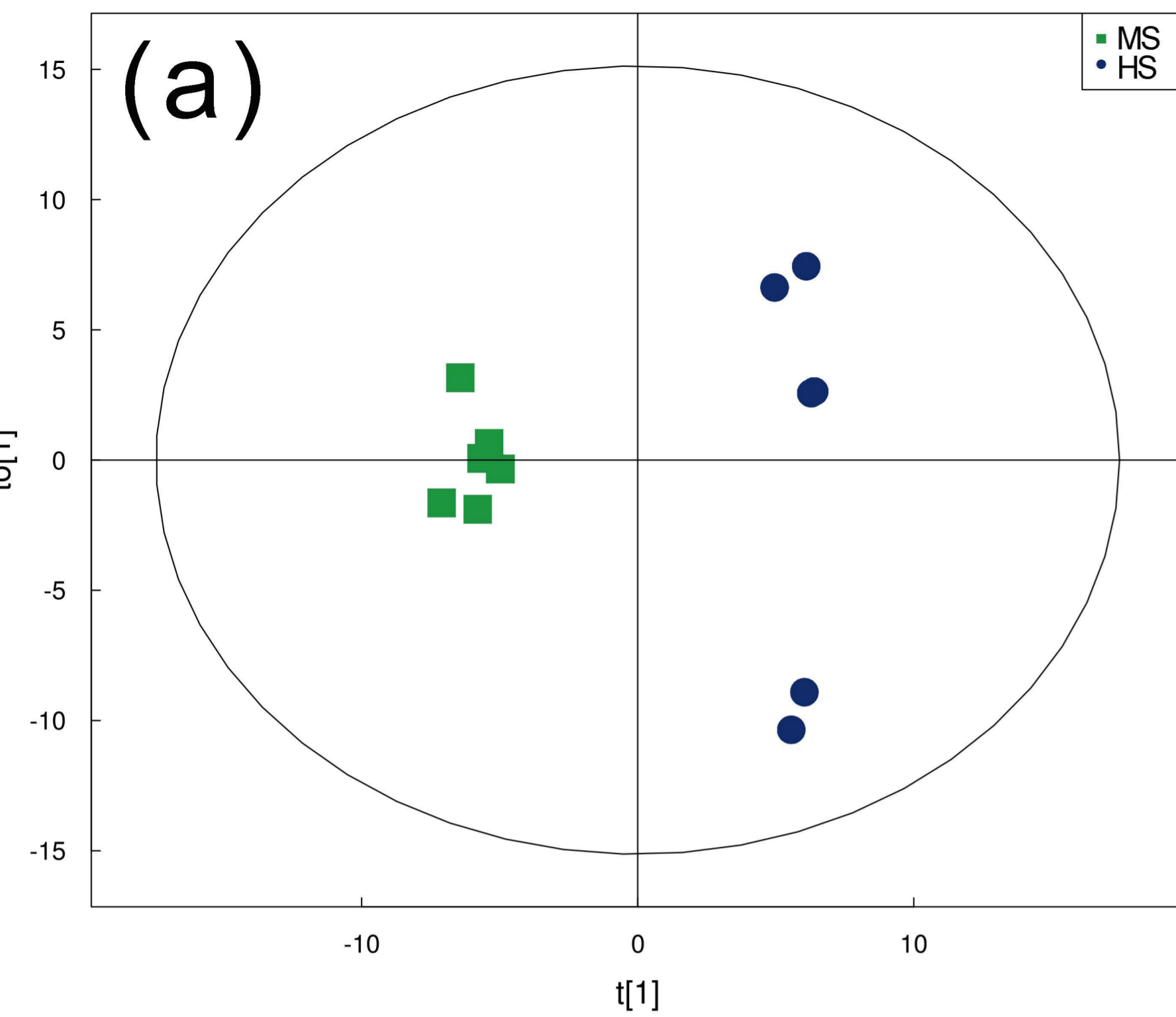
Scores (OPLS-DA)
