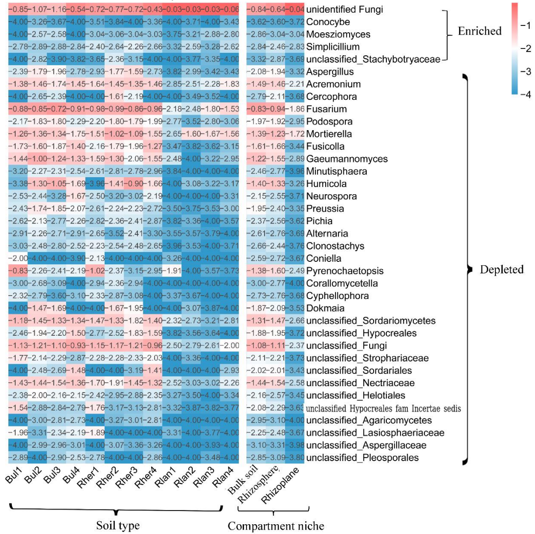
heatmap
