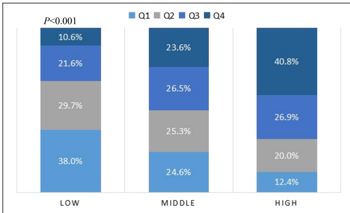
Supplemental Figure 1. The distribution of AIP levels in different BMI groups.
