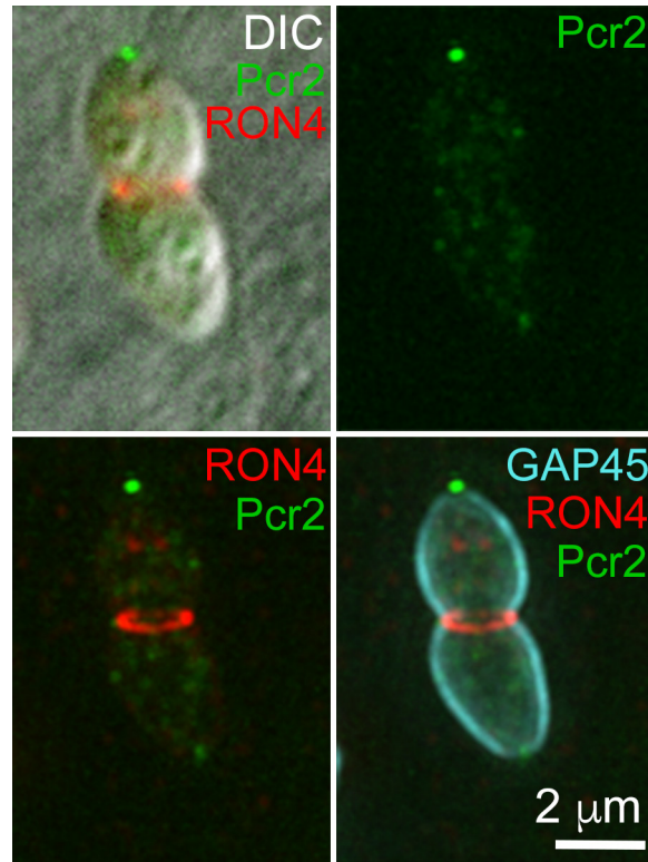
S2 Fig. DIC and projections of deconvolved wide-field fluorescence images of an invading Pcr2-mNeonGreen 3' tag parasite (green), in which the moving junction (anti-RON4, red), and the parasite cortex (anti-GAP45, cyan) were labeled by immunofluorescence.
