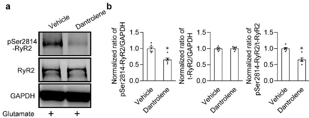
Fig. S6. Dantrolene decreased the glutamate-induced RyR2 phosphorylation in rat SANPCs.
