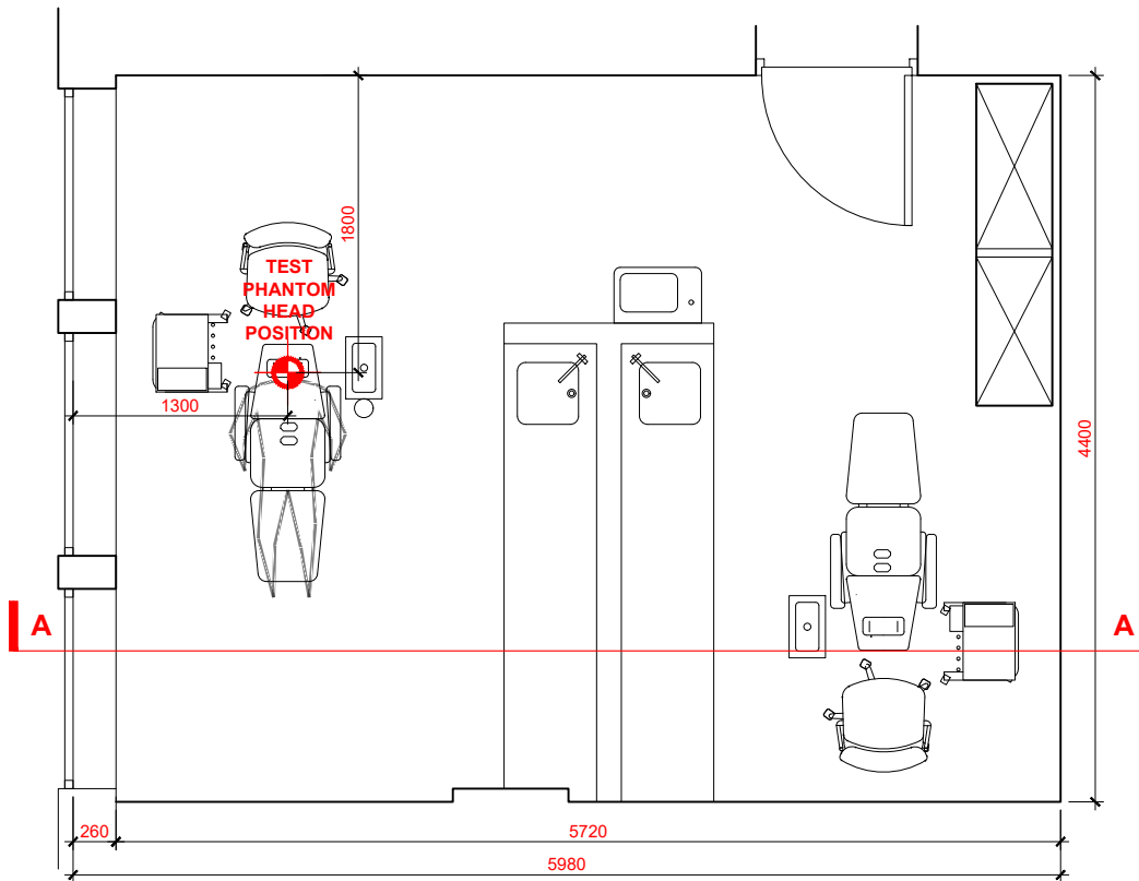
PLAN VIEW
