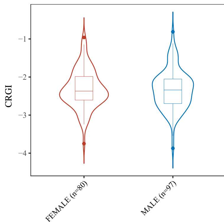
Kruskal-Wallis test p=0.35
