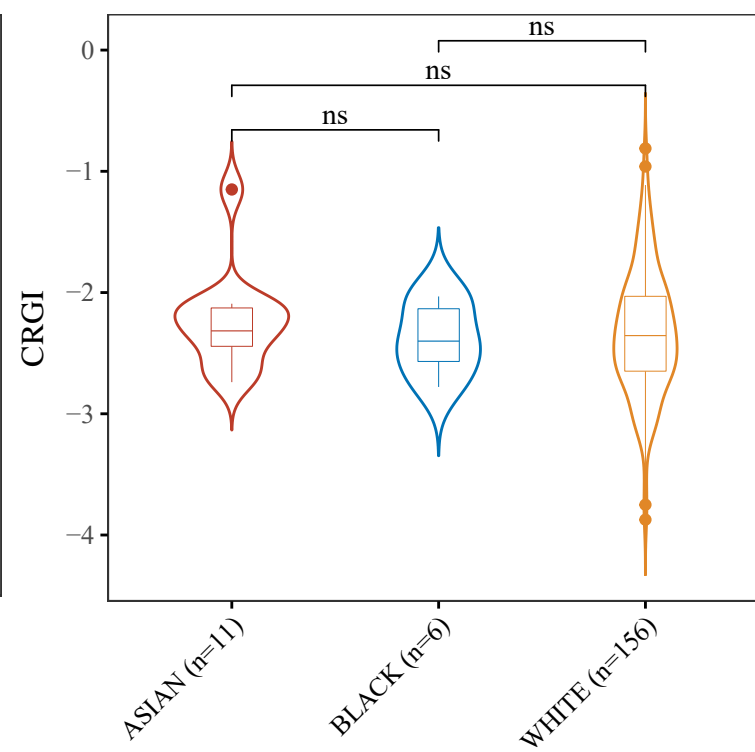
Kruskal-Wallis test p=0.21
