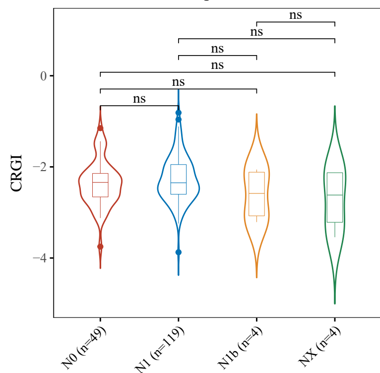
Kruskal-Wallis test p=0.19
