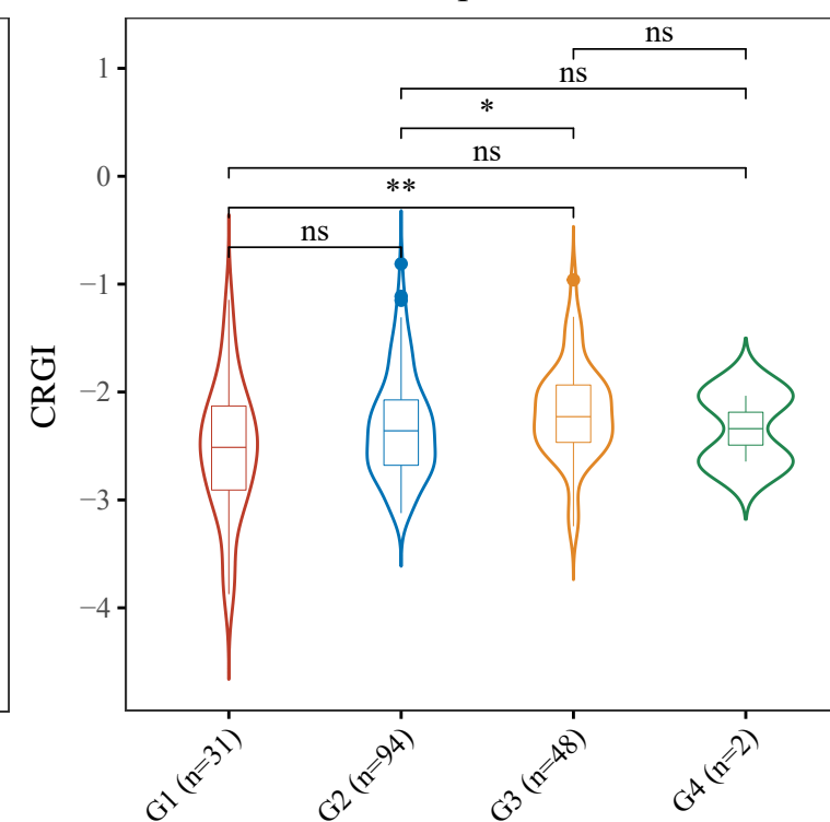
Kruskal-Wallis test p=0.028
