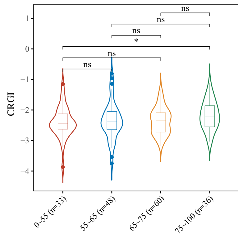
Kruskal-Wallis test p=0.36
