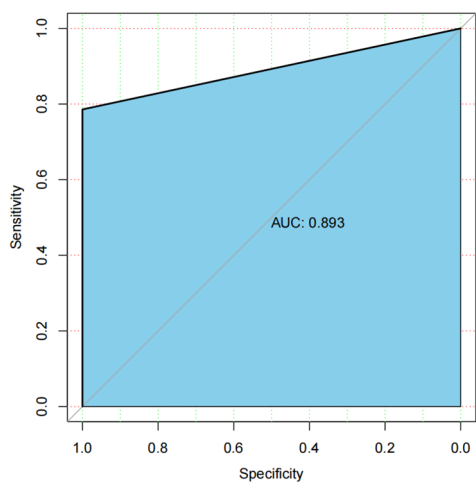
Figure S3 ROC curve.
