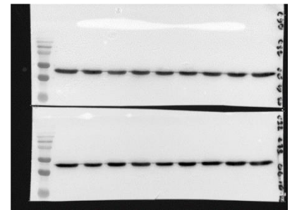
Actin
