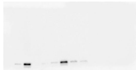
Mcl1
