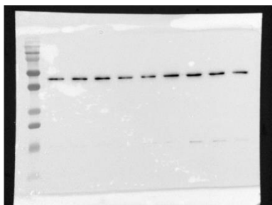
Actin
