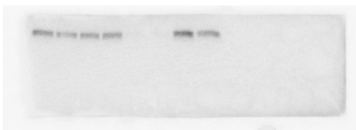
actin
