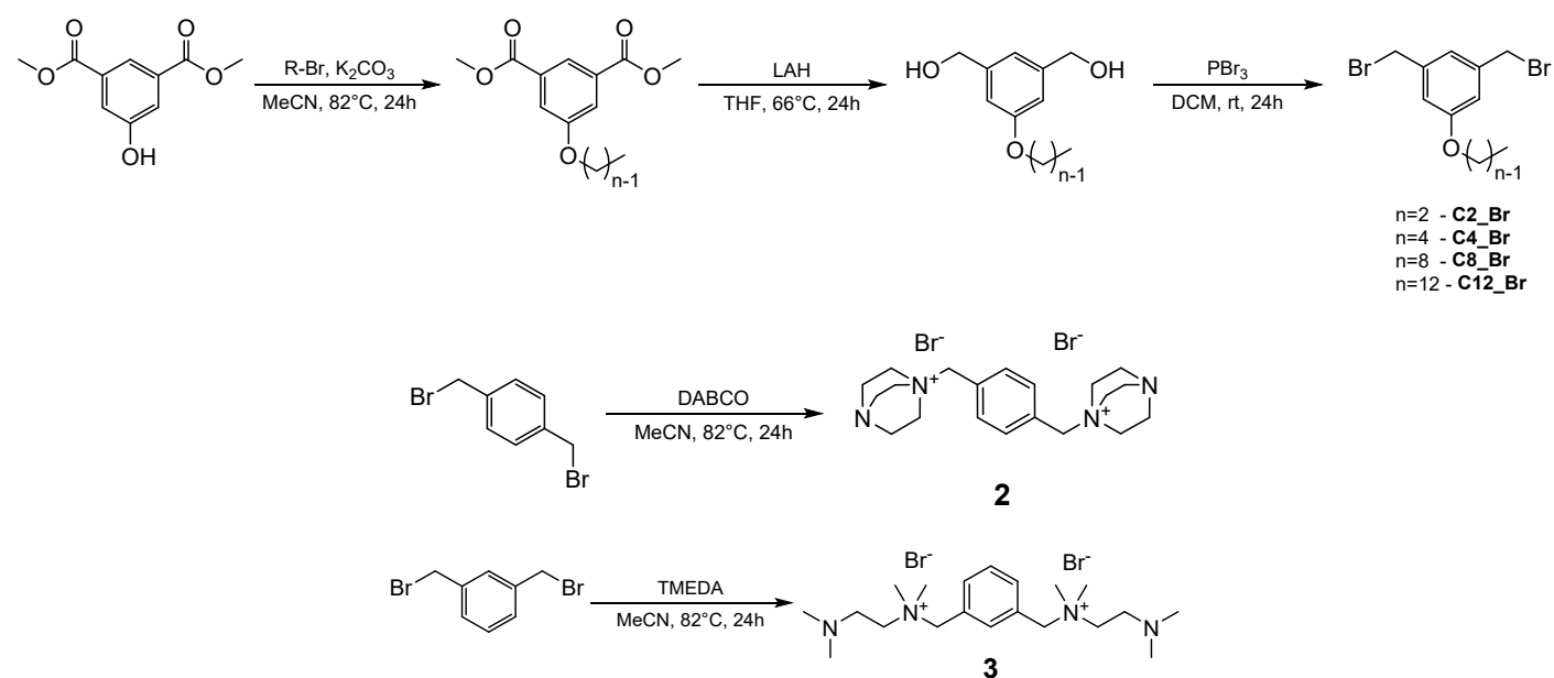
Scheme S1. The synthesis of used monomers in the ionenes synthesis.
