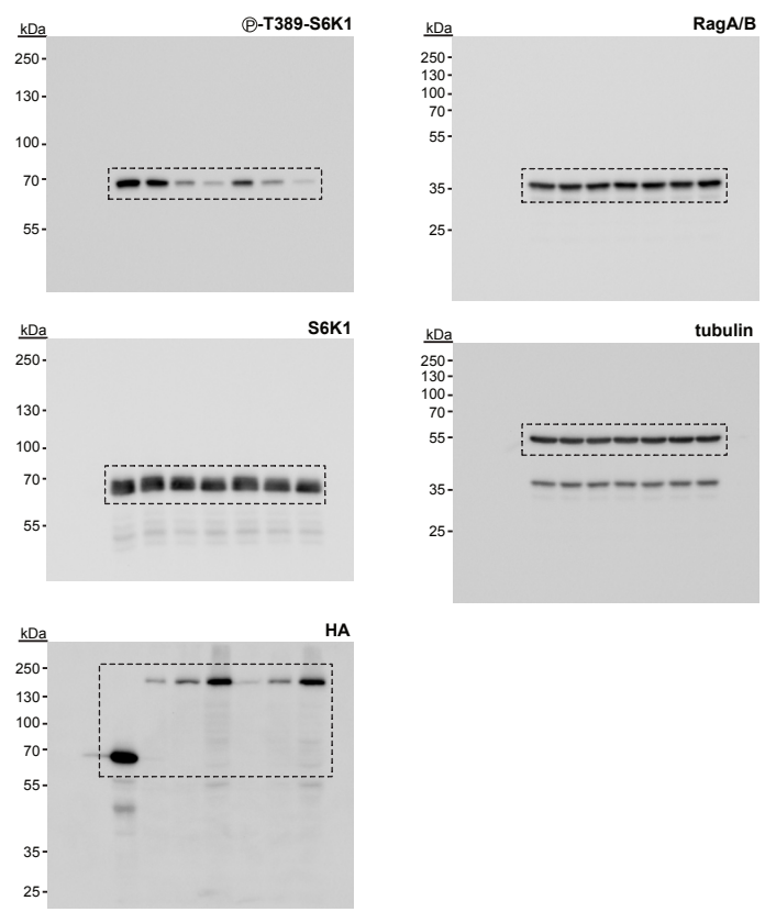
Fig. 3c unprocessed blots
