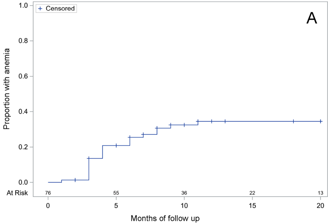
Supplemental Figure 1. Cumulative proportion of patients with incident anemia (A) and thrombocytopenia (B) during linezolid therapy for MDR-TB.
