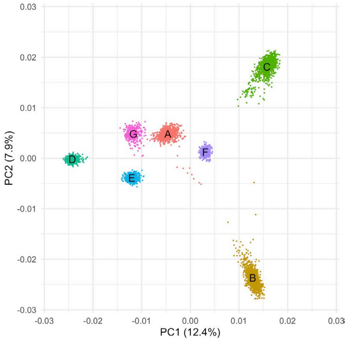
Figure S1. Population structure of the sequenced pigs according to the two first principal components. The colour clusters correspond to lines A to G.
