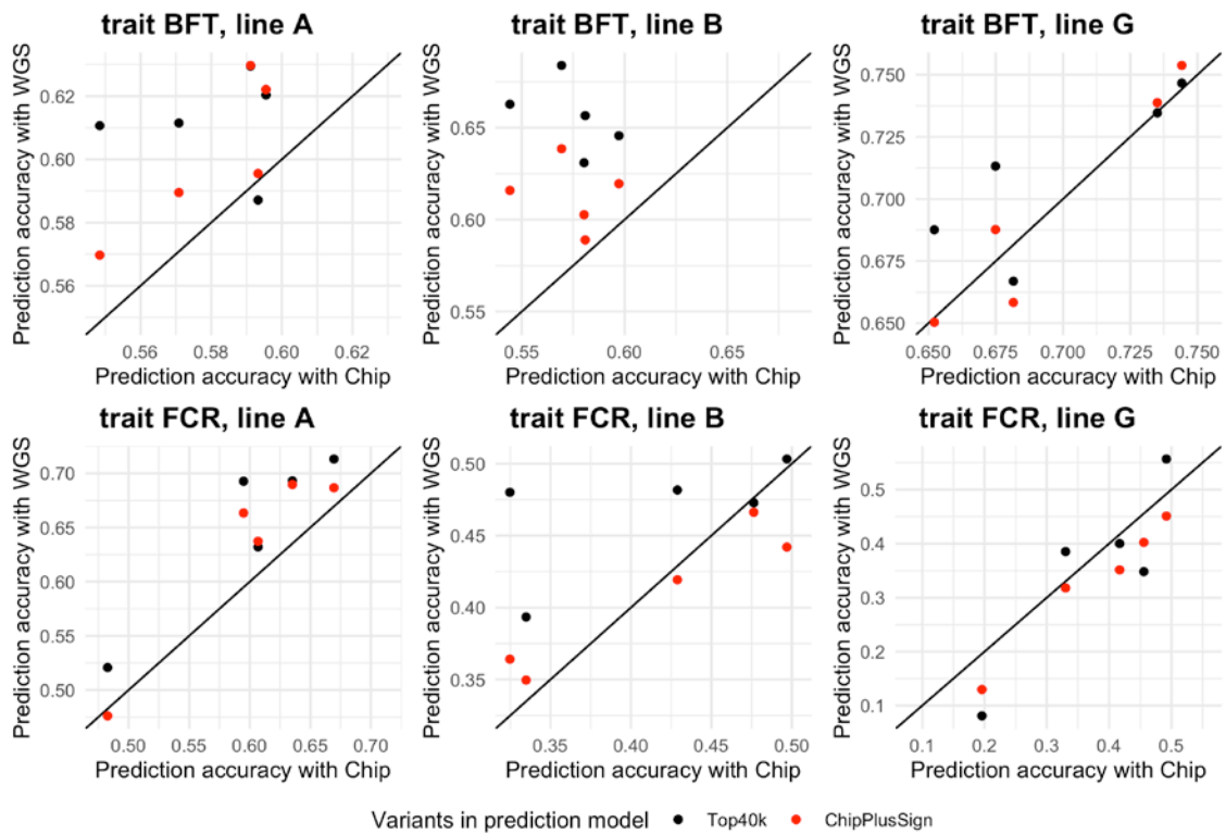
Figure S3. Genomic prediction accuracy obtained with each set of preselected whole-genome sequence (WGS) variants (either Top40k or ChipPlusSign) against that obtained with the marker array (Chip) in each of the five replicates.
