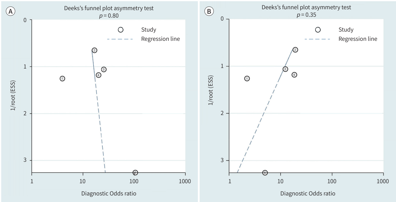
Supplementary Fig. 3. Deeks' funnel plot to evaluate publication bias regarding LI-RADS treatment response (A) and mRECIST viable category (B). ESS = effective sample size, LI-RADS = Liver Imaging Reporting and Data Systems, mRECIST = modified Response Evaluation Criteria in Solid Tumors
