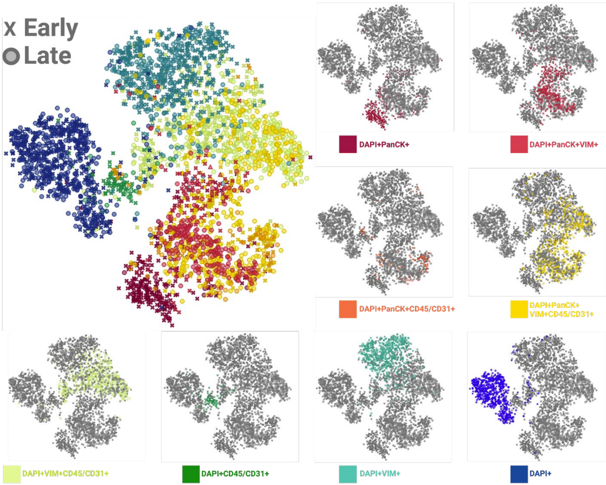
Supplementary Figure 1. Visualization of rare cell features. T-SNE embedding of rare cells based on morphometric features derived from OCULAR. Each designated color represents a classification group marked in the figure.
