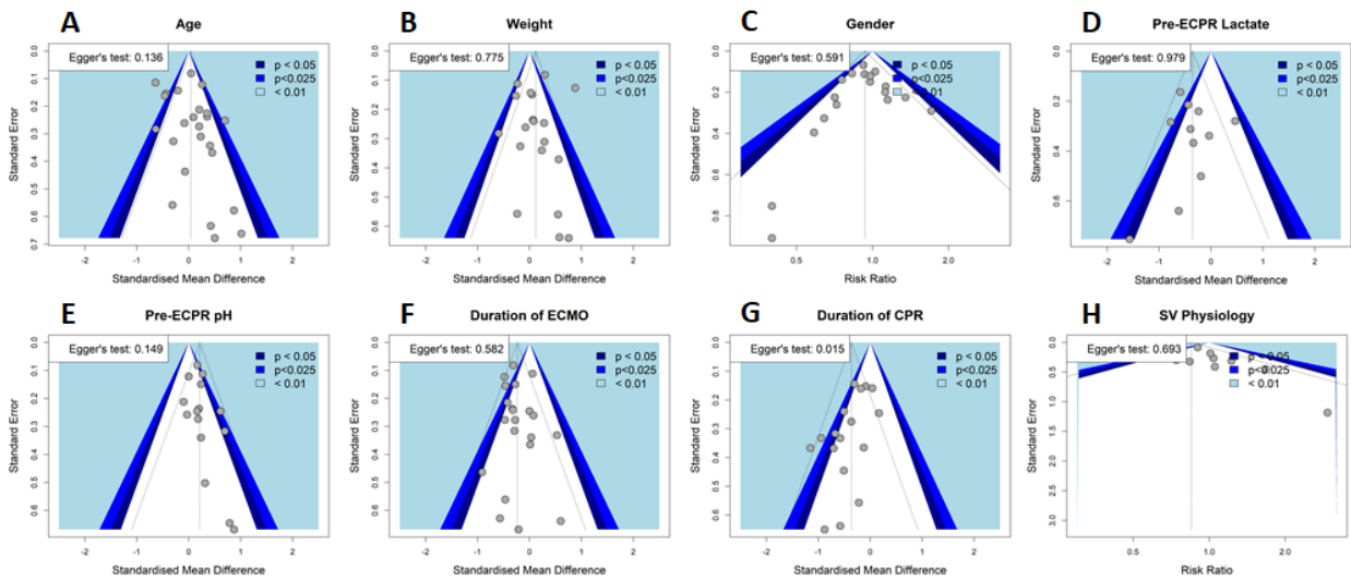
Supplemental Figure 2. Funnel plots examining publication bias in Patient Demographics Metrics. (A) Age, (B) Weight, (C) Gender, (D) pre-ECPR lactate, (E) pre-ECPR pH, (F) Duration of ECMO, and (G) Duration of CPR, and (H) Single Ventricle Physiology. Egger's tests were additionally conducted and are displayed in the top left of each funnel plot. No publication bias was detected in any metric except duration of CPR.
