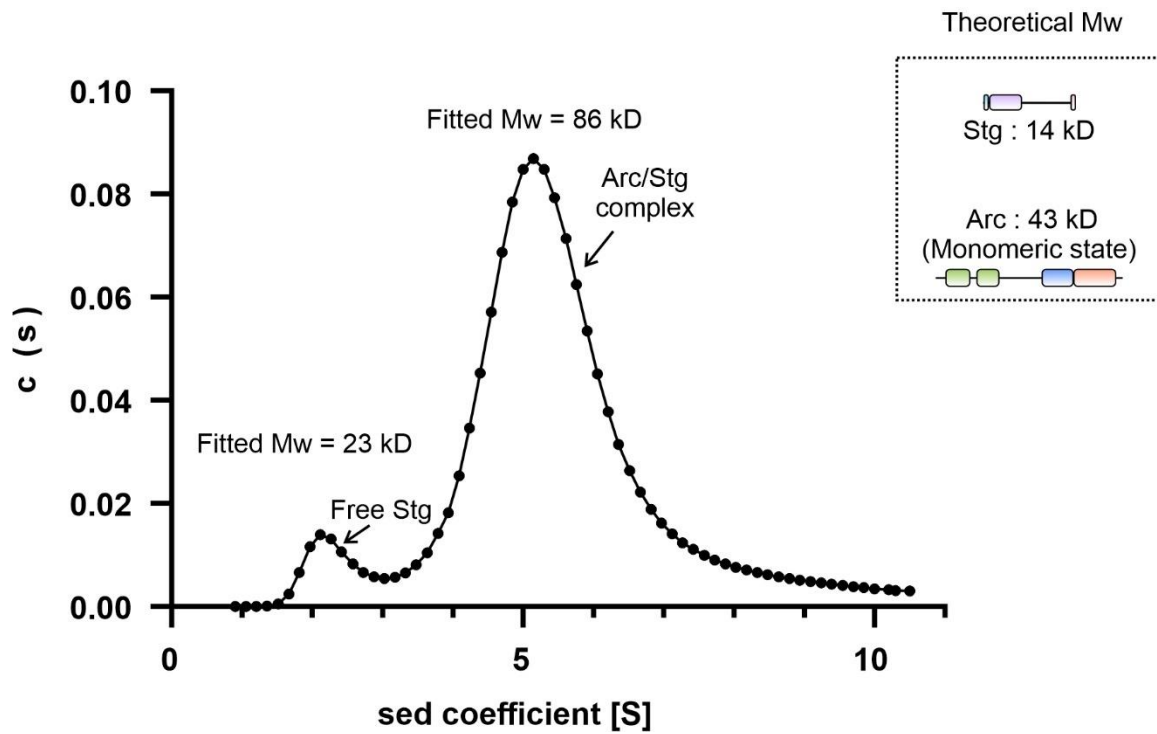
Supplementary information, Fig. S10: Arc and Stg do not form high ordered protein assembly. The analytical ultracentrifugation analysis showing the Arc and Stg failed to form large protein assembly. 5 \mu M Arc was mixed with 15 \mu M Stg. The fitted molecular masses are shown in plot, and theoretical molecular masses are presented in the box.
