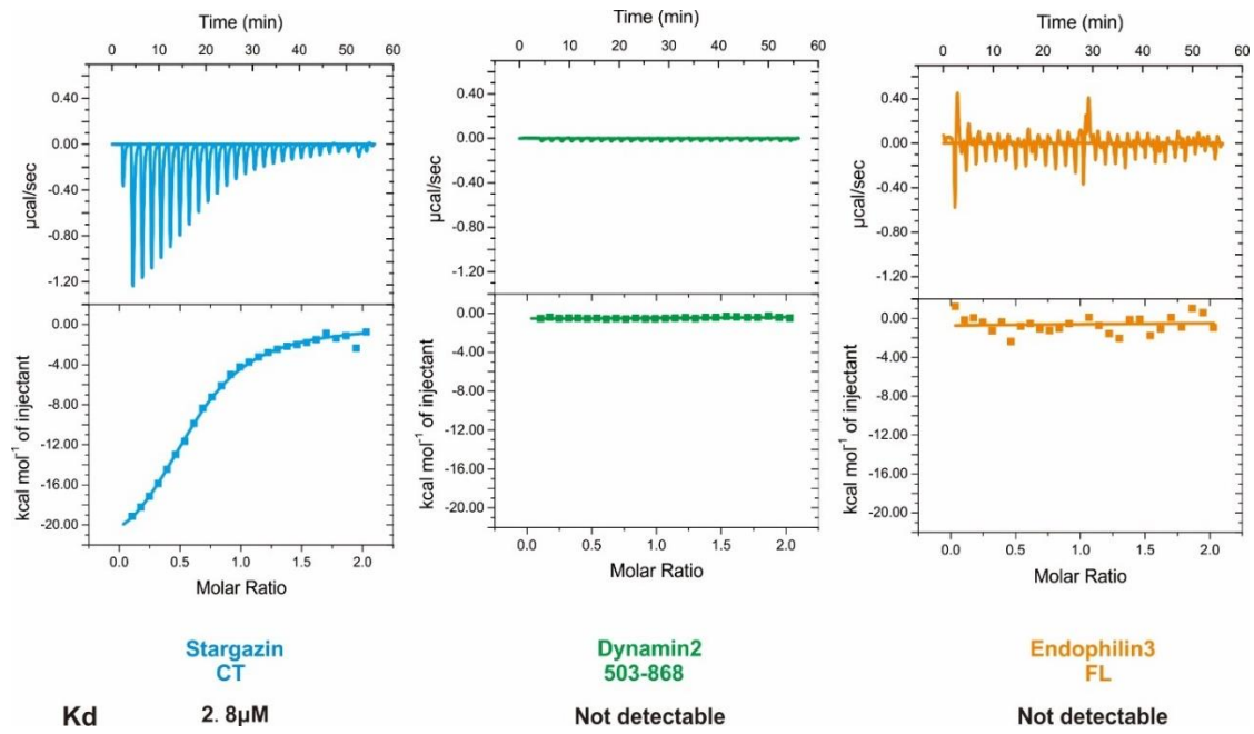
Supplementary information, Fig. S9: ITC measurement detecting binding between GAG domain of Arc and Stargazin CT/ Dynamin2/ Endophilin3. 200 \mu\text{M} Stg-CT, Dynamin2 (a.a. 503-868) or Endophilin3 in the syringe was titrated to 20 \mu\text{M} GAG domain of Arc.
