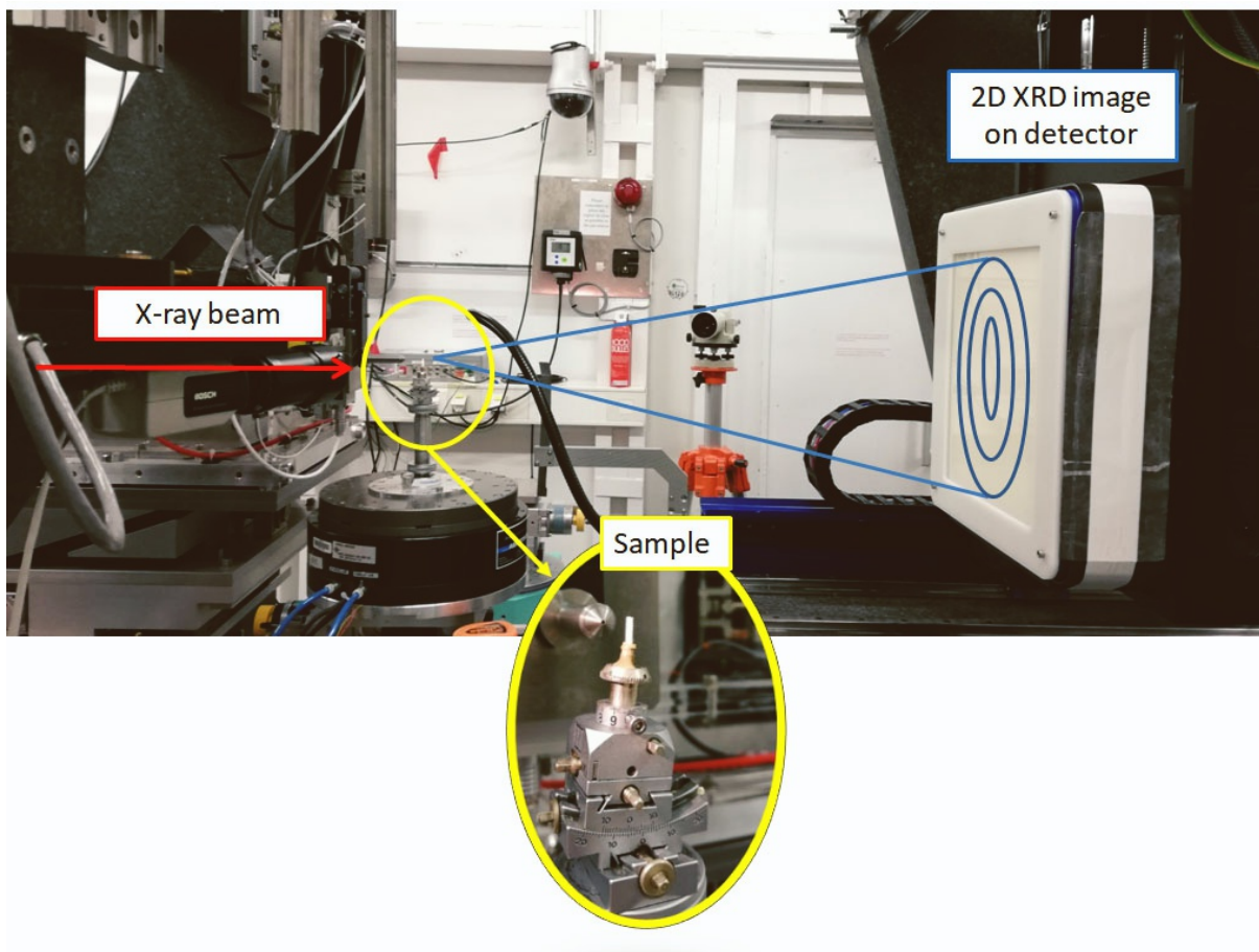
Figure S1. XRDCT experimental setup (ID15a beamline, ESRF) used for the Noto limestone experiment, Related to STAR Methods
