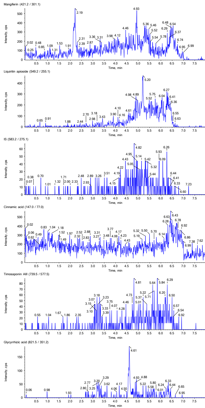
Figure S3. The chromatogram of selectivity of the analytes in rat serum: blank serum sample (a), blank serum sample spiked with standard compounds (b), and a serum sample obtained from a rat at 2h after BHGZD gavage (c).
