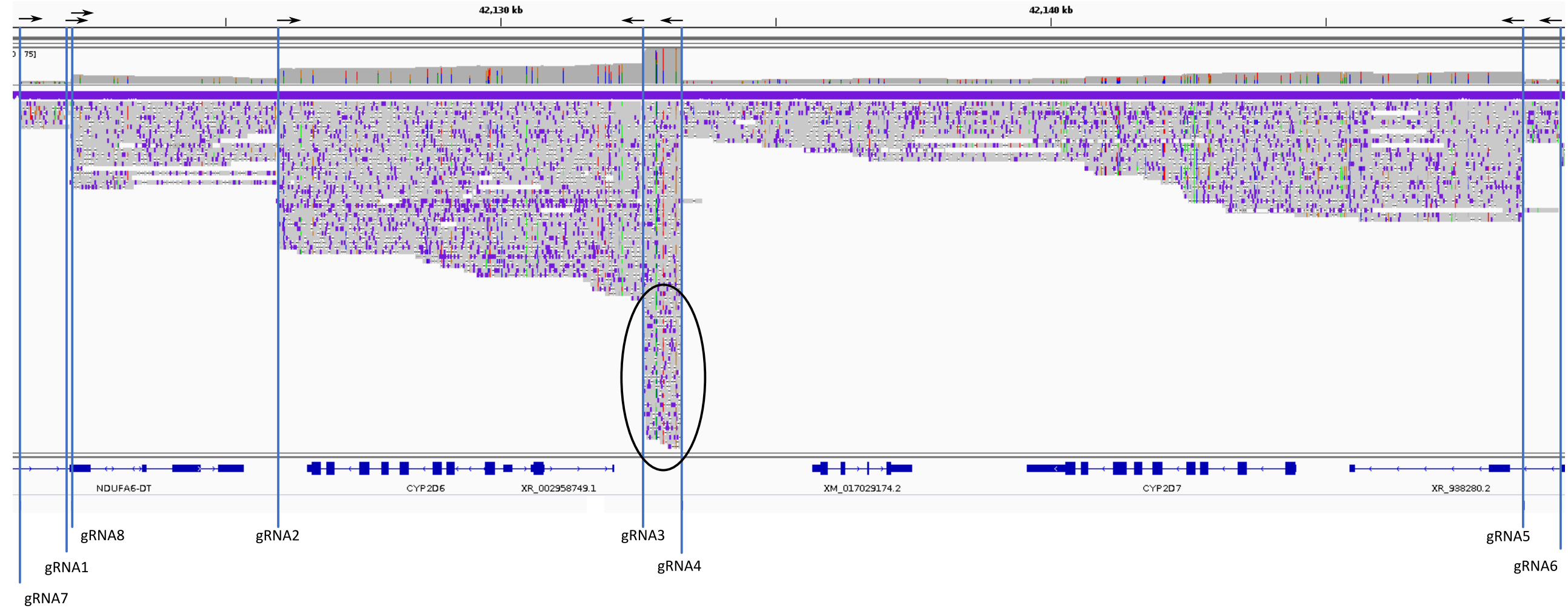
S3 Fig Reads of the NA12878 DNA, sequenced on a Flongle flow cell, mapped on the GRCh38 reference genome. The positions of the gRNAs are indicated with vertical lines and the sequencing direction is indicated with arrows on top of the vertical lines. gRNA3 cut reads generated by gRNA4, causing a lower depth on CYP2D6 .
