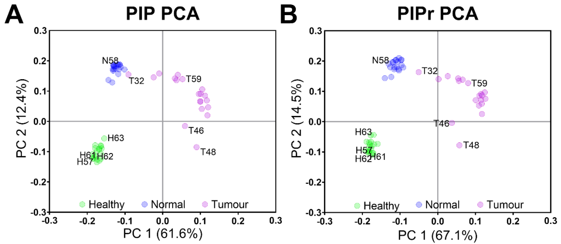
Figure S1. Principal components analysis (PCA) of peptide (A) and protein (B) similarity data. Analysis was based on percentage identical peptide (PIP) and percentage identical protein (PIPr) values, respectively.
