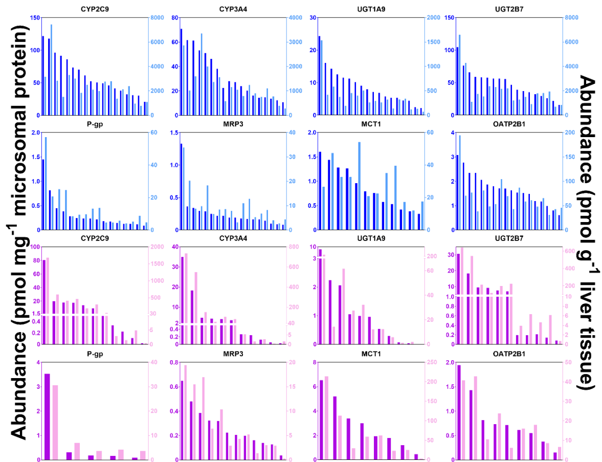
Figure S2. Abundance of CYP2C9, CYP3A4, UGT1A9, UGT2B7, P-gp, MRP3, MCT1, and OATP2B1 in histologically normal (graphs on the top, blue bars) and tumour (graphs at the bottom, purple bars). Abundance is expressed in pmol of target protein per mg of microsomal protein on the left y-axis (darker bars), and as pmol of target protein per g of liver on the right y-axis (lighter bars).
