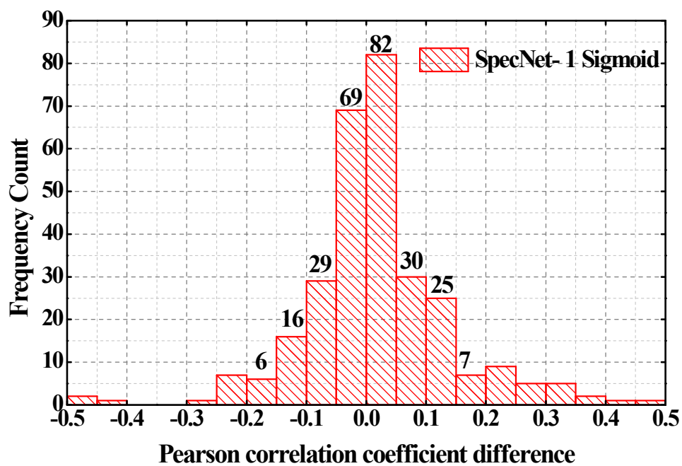
Fig. 1 Histogram plot of the PCC difference obtained from the SpecNet and 1 Sigmoid model.
