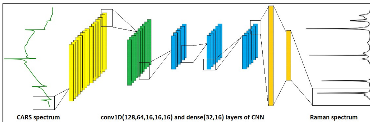
Fig. 2 Typical schematic of the CNN model architecture.
