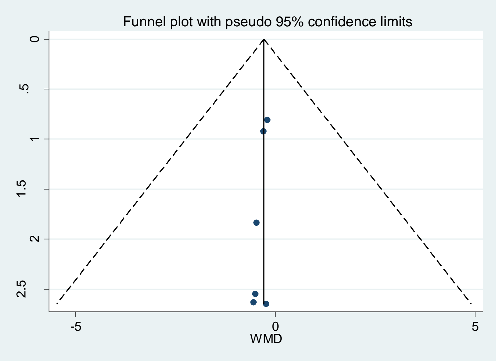
Supplementary Figure 1. Funnel plot to assess publication bias.
