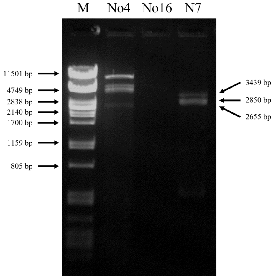
Fig. ESM1: 1 % agarose gel with dsRNA of different fungal isolates. Lines: M: DNA ladder (Phage lambda DNA, PstI digested); No4: Rugonectria rugulosa ; No16: Dactylonectria torresensis , N7: Ilyonectria pseudodestructans .
