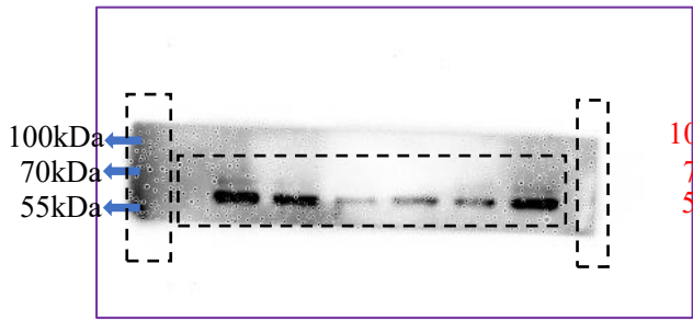
CTSB 27KDa
