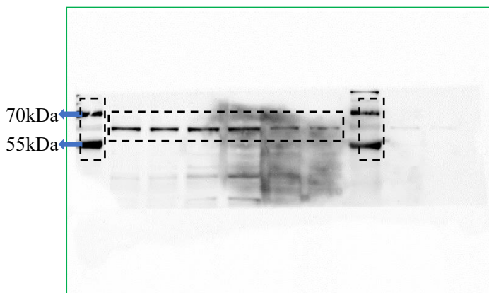
p-TFEB 62KDa
