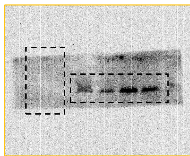
GAPDH 37KDa
