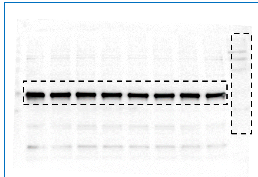
GAPDH 37KDa
