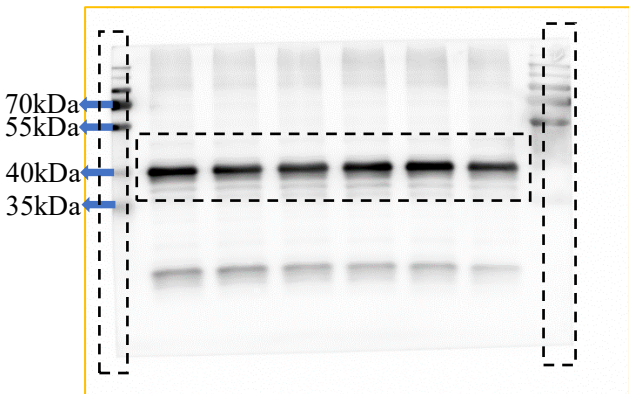
GAPDH-37KDa
