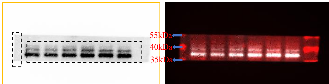
GAPDH 37kDa
