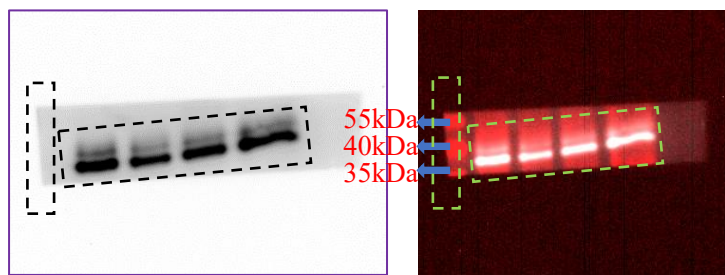
GAPDH 37KDa
