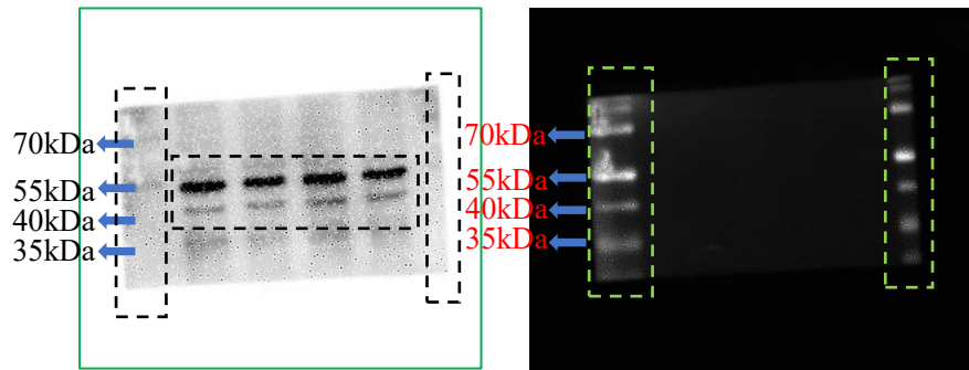
mTOR 289KDa
