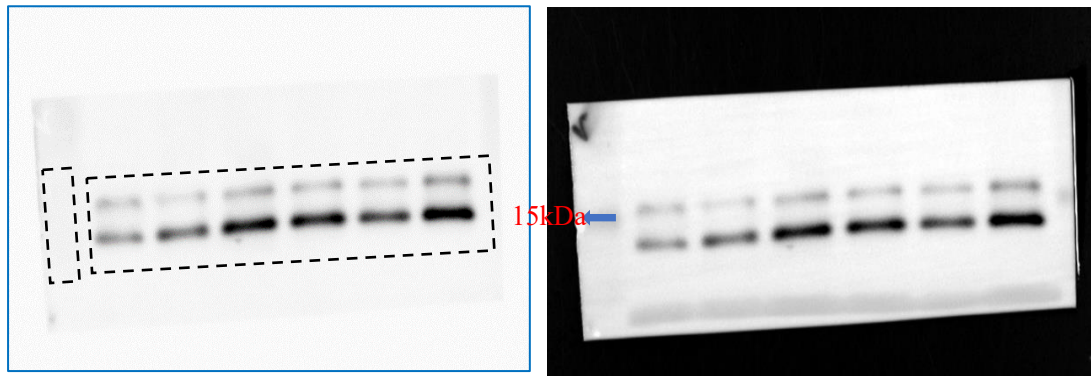
GAPDH 37kDa
