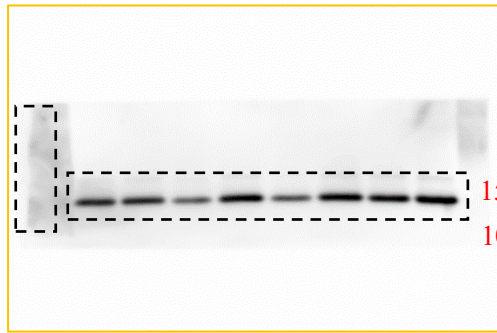
GAPDH 37KDa
