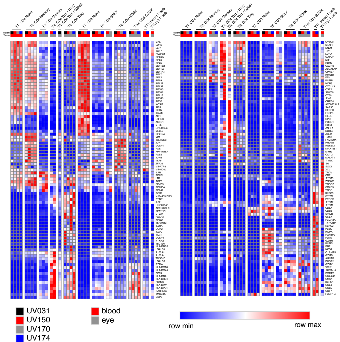
Supplemental Figure 7: Expanded T cell cluster gene expression reveals shared and unique genes for each T cell cluster. Cluster-associated relative gene expression for indicated patient and tissue.
