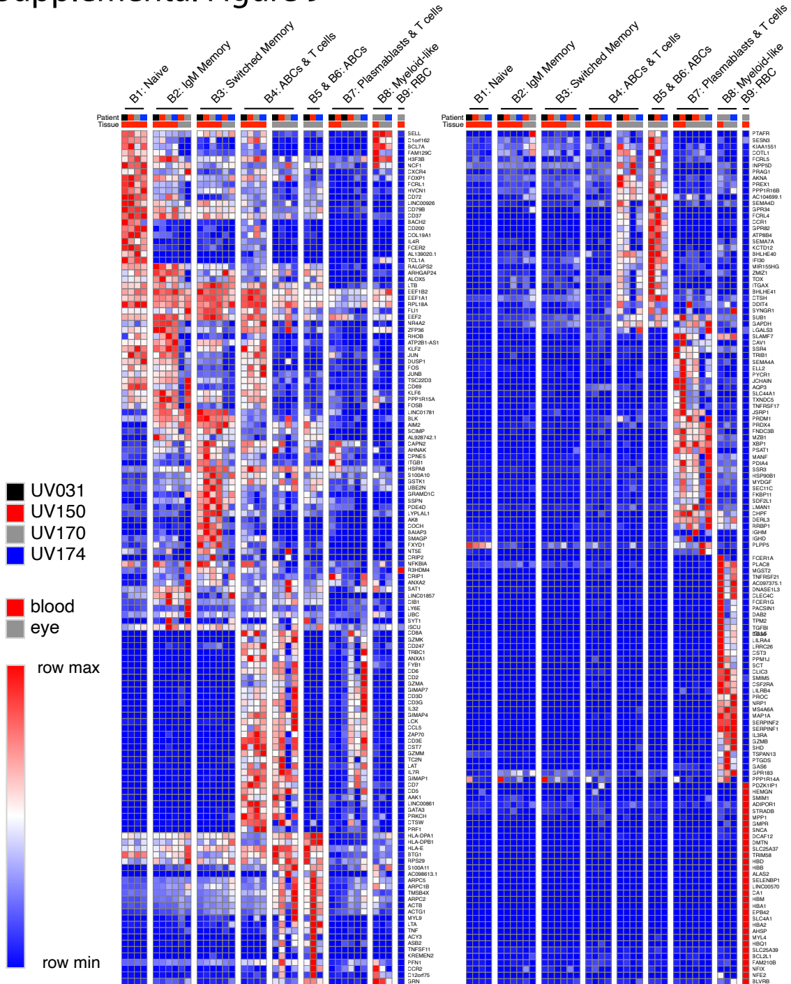
Supplemental Figure 9: Expanded B cell cluster gene expression reveals shared and unique genes for each B cell cluster. Cluster-associated relative gene expression for indicated patient and tissue.
