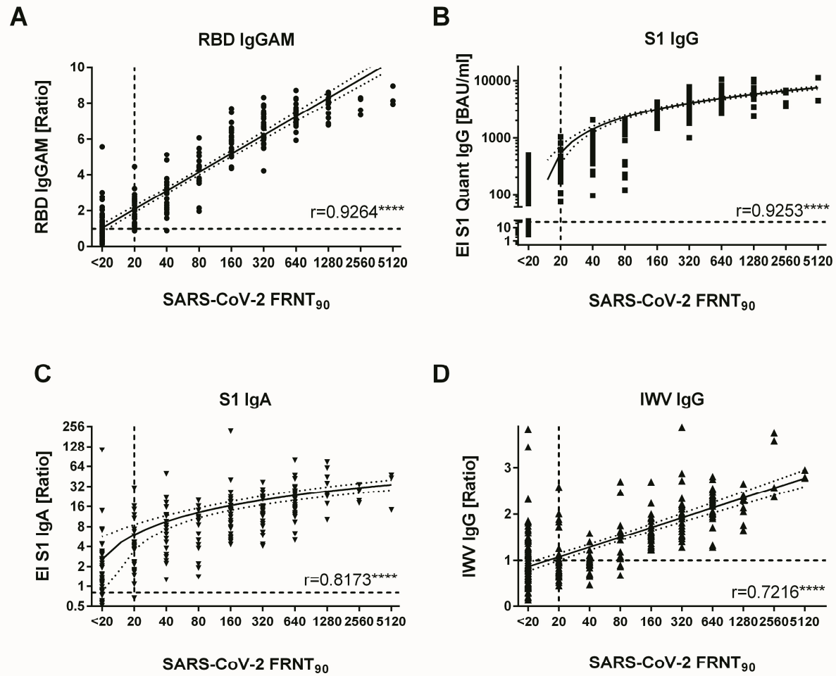
S1 Fig: Correlation between different BNT162b2-induced antibodies and SARS-CoV-2 virus neutralizing titers. Horizontal dotted line represents the cut-off values of the ELISAs. The vertical dotted lines show the neutralization assay cut-off. (A) RBD IgGAM as sample/calibrator ratio (B) S1 IgG antibodies were measured quantitatively [BAU/ml] (C-D) IWV IgG and S1 IgA antibodies are depicted as sample/calibrator ratios.
