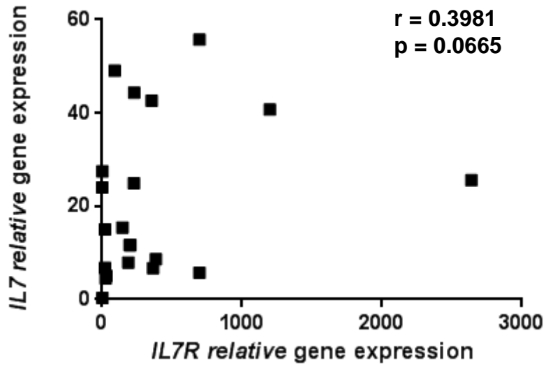
Supplementary figure 2: Correlation between IL7 and IL7R mRNA expression in MPM cells. mRNA expression was measured using RT-PCR. Correlation was analyzed using non-parametric Spearman test.
