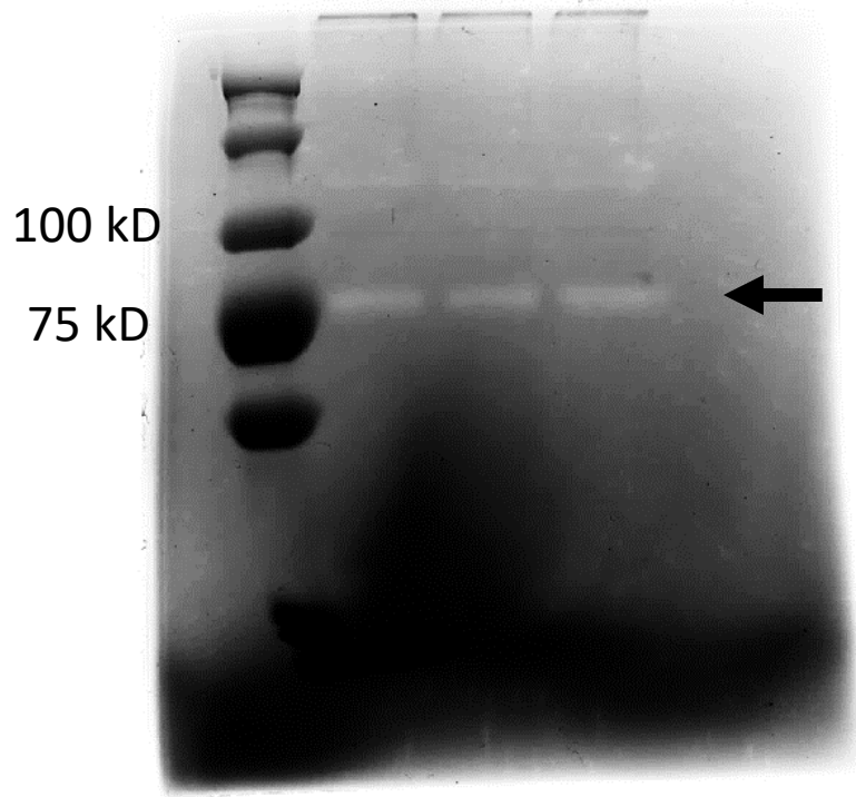
Gelatin zymography
