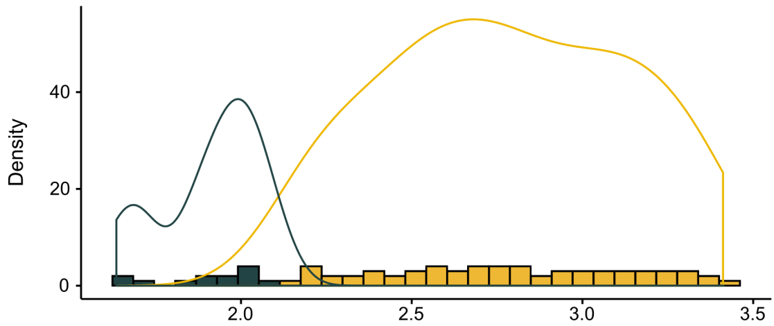
Maximally selected rank statistics
