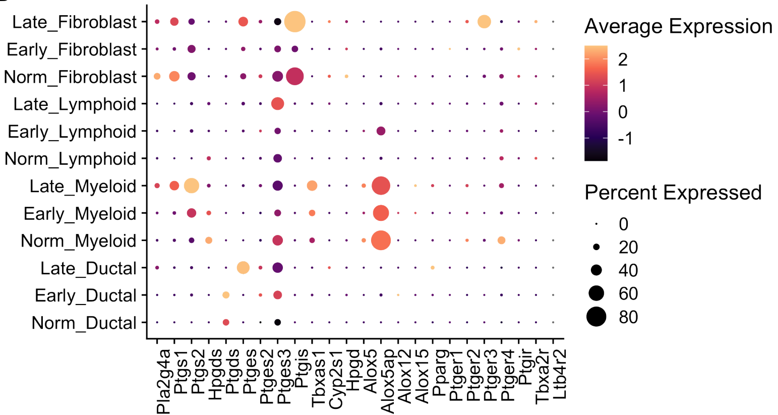
Figure S2. Eicosanoid pathway gene expression in multiple murine models of PDAC. Dotplots of eicosanoid synthase and receptor gene expression in normal pancreas and tumor epithelium organized by (A) mouse model or (B) stage of disease progression from the datasets described in Hosein et. al. KPC, LSL-KrasG12D;Trp53R172H;Ptf1aCre/+; KIC, LSL-KrasG12D; Ink4af1/fl;Ptf1aCre/+; KPFC, LSL-KrasG12D;Trp53fl/fl; Pdx1Cre/+. Norm, normal; Early, early lesions; Late, PDAC.
