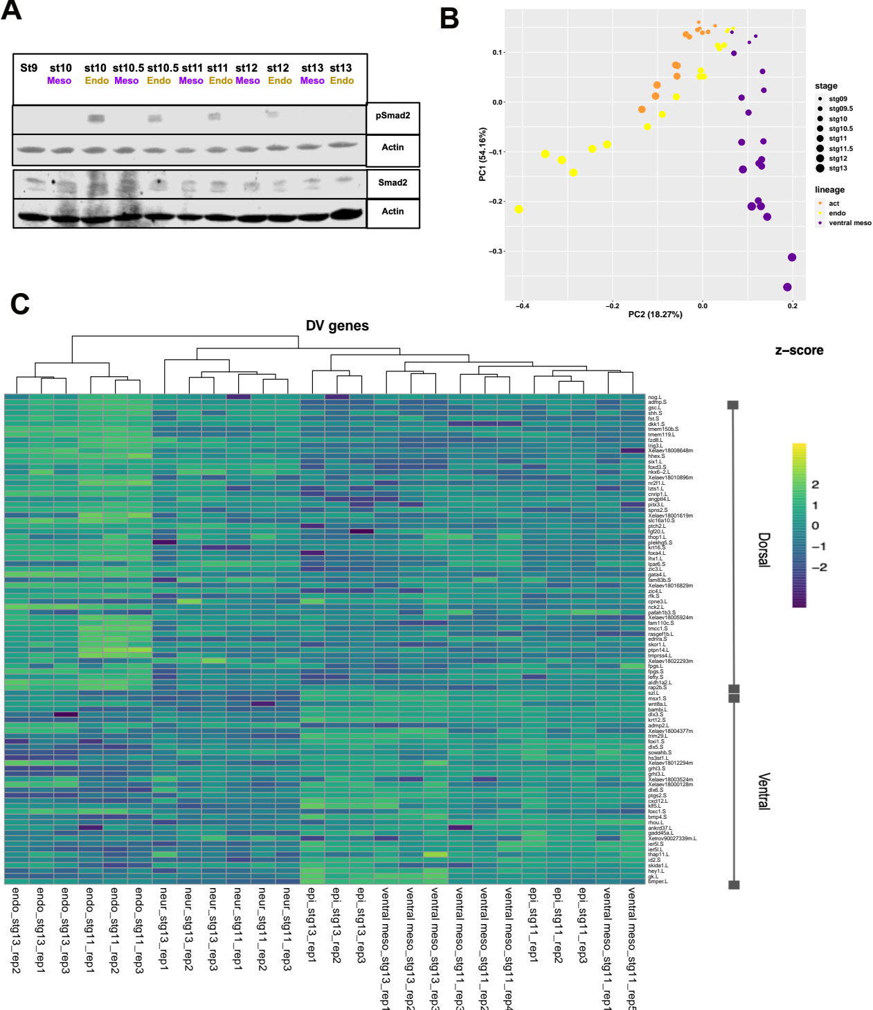
Supplemental Figure 5. BMP Ventralizes Mesoderm. (A) Western blot analysis of lysates of developing mesoderm (20ng/uL BMP4/7) and endoderm (160ng/uL Activin) explants for pSmad2 and Smad2 with Actin loading control. Gels were cropped to minimize empty space, uncropped gels are Supplemental Figure 9A. (B) PCA of published Activin induced mesoderm data (Satou-Kobayashi et al. 2021) with our ventral mesoderm and endoderm data shows that activin induced mesoderm clusters with our activin induced endoderm rather than BMP4/7 induced mesoderm. (C) Hierarchical clustering of Dorsal/Ventral genes (Ding et al. 2017) shows that endoderm and ventral mesoderm cluster on opposite sides of the heat map, suggesting BMP4/7 effectively ventralizes the mesoderm.
