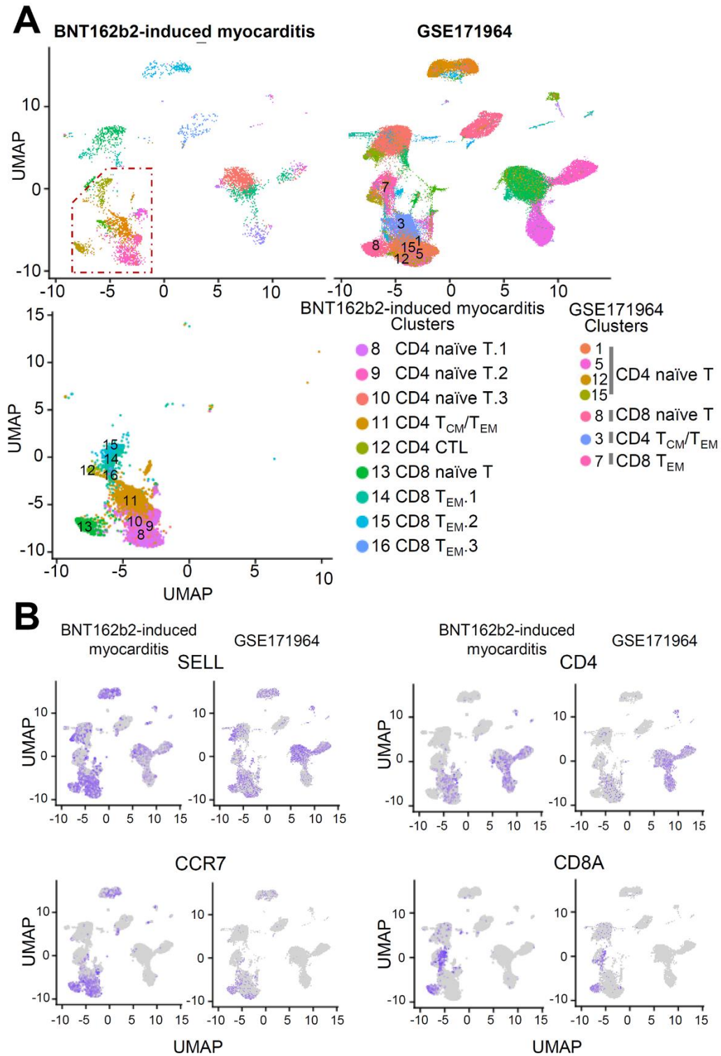
Supplementary Fig. S1. T cell subpopulations of PBMCs of vaccinated individuals and BNT162b2-induced myocarditis patient. (A) T cell clusters of GSE171964 are identified after integration with BNT162b2-induced myocarditis data. (B) Feature plot showing distribution of T cell markers.
