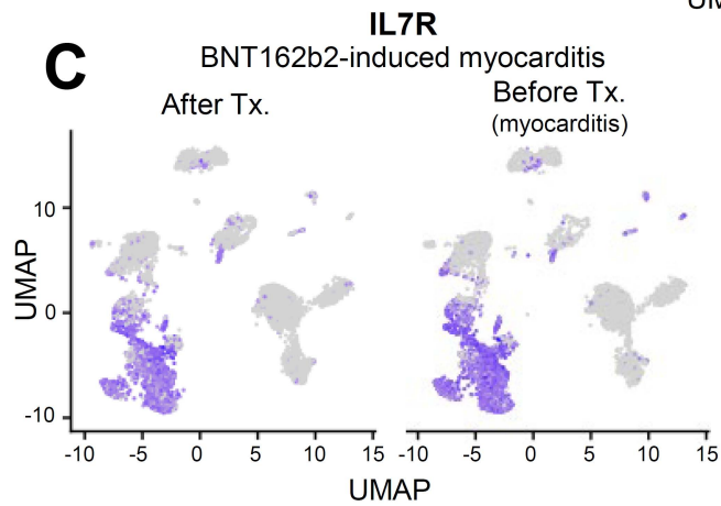
Supplementary Fig. S2. Up-regulation of IL7R mRNA expression level in BNT162b20-induced myocarditis patient. (A) Volcano plot of differentially expressed genes with adjusted P value less than 0.1. (B) Feature plot showing IL7R distribution in GSE171964. (C) Feature plot showing IL7R distribution in this data.
