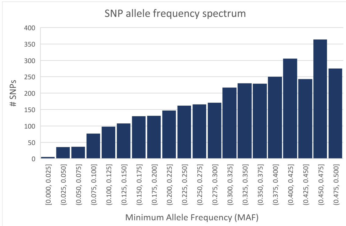
Supporting File S3. Site frequency spectrum of the 3380 SNPs in the 90 Theobroma cacao clones studied.
