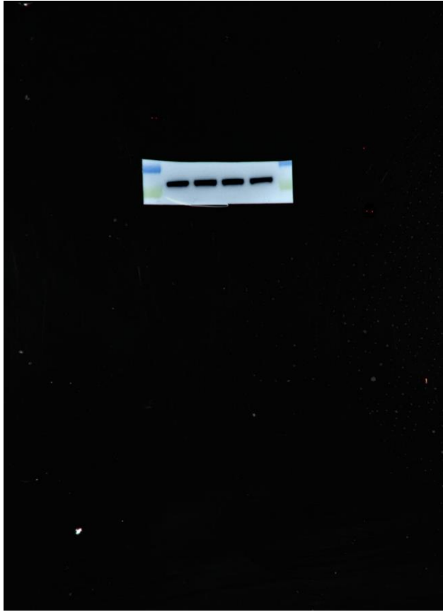
Full unedited blot for Figure 3D GAPDH
