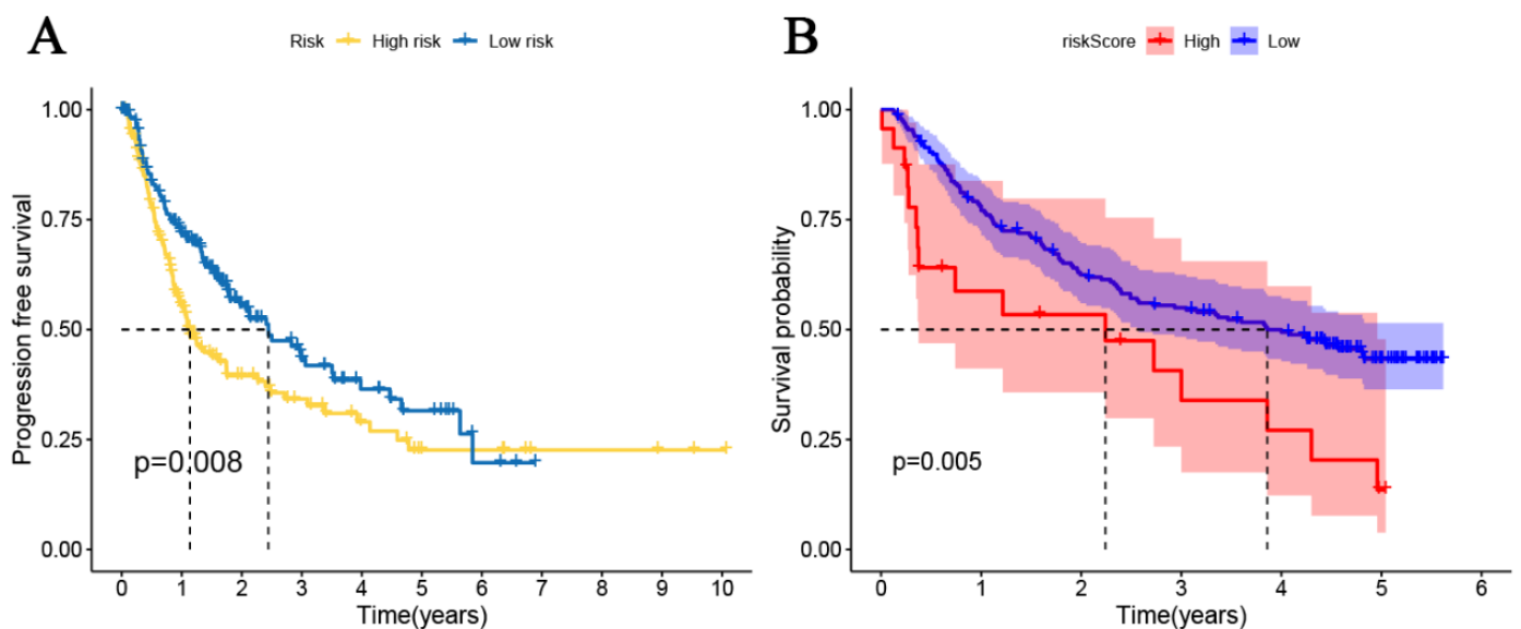
Figure S2. PFS value of (A) TCGA-HCC dataset and (B) GSE14520 dataset.
