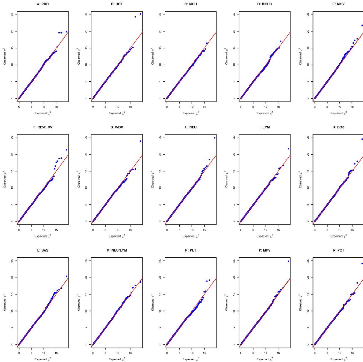
Supplementary Figure 1. Quantile-quantile (Q-Q) plots of genome-wide association studies (GWAS) after correcting p-values for the relevant traits. Red blood cell (A), Hematocrit (B), Mean corpuscular hemoglobin (C), Mean corpuscular hemoglobin concentration (D), MCV: Mean corpuscular volume (E), RBC volume distribution width coefficient of variation (F), White blood cell (G), Neutrophils (H), Lymphocytes (I), Eosinophils (K), Basophils (L), neutrophils/lymphocytes (M), Platelets (N), Mean platelets volume (P), Procalcitonin (R).
