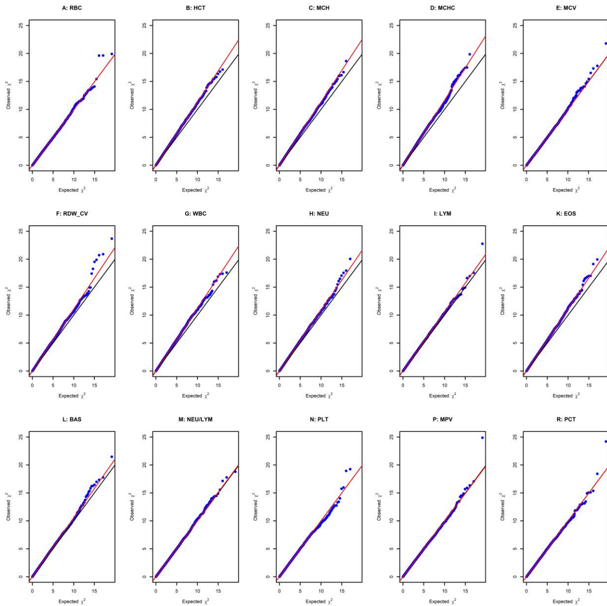
Supplementary Figure 3. Quantile-quantile (Q-Q) plots of genome-wide association studies (GWAS) before correcting p-values for the relevant traits. Red blood cell (A), Hematocrit (B), Mean corpuscular hemoglobin (C), Mean corpuscular hemoglobin concentration (D), MCV: Mean corpuscular volume (E), RBC volume distribution width coefficient of variation (F), White blood cell (G), Neutrophils (H), Lymphocytes (I), Eosinophils (K), Basophils (L), neutrophils/lymphocytes (M), Platelets (N), Mean platelets volume (P), Procalcitonin (R).
