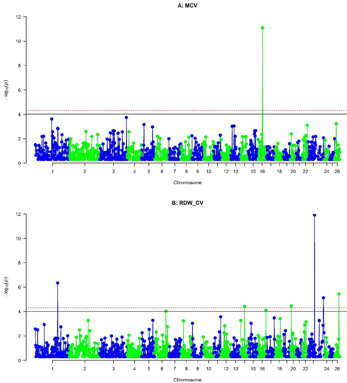
Supplementary Figure 4. Manhattan plots for associations between regions and mean corpuscular volume (MCV) and RBC volume distribution width coefficient of variation (RDW_CV). Red dashed horizontal lines indicate suggestive (0.10) significance and black horizontal line indicate genome-wide (0.05) significance with 1,038 windows.
