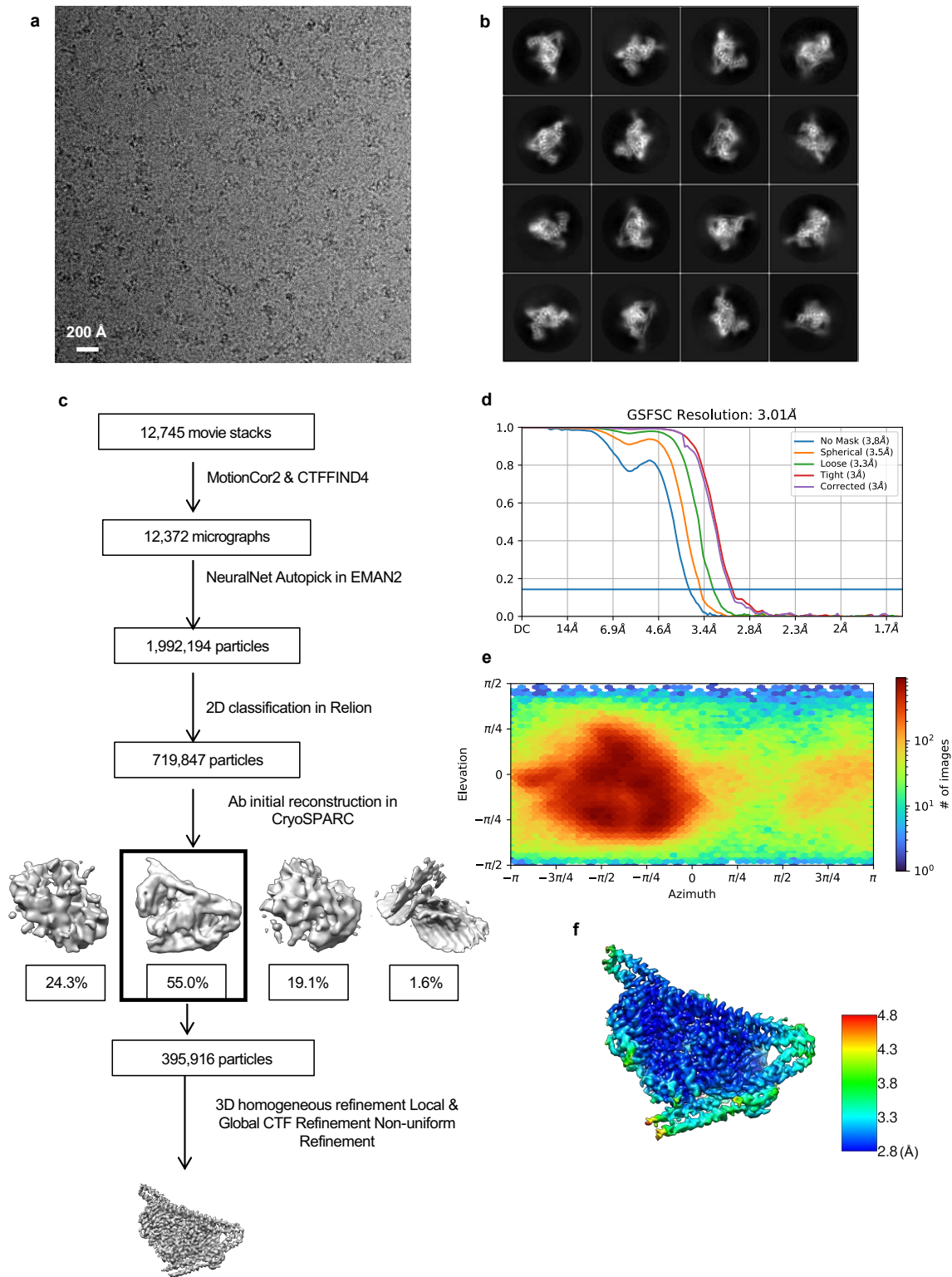
Supplementary information, Fig. S1. Single-particle cryo-EM analysis of the HWVZ complex. a Representative motion-corrected cryo-EM micrograph. b Reference-free 2D class averages. c Workflow of the data processing. d Gold standard FSC plots calculated in cryoSPARC. e Euler angle distribution of the particle images. f Resolution map for the final 3D reconstruction.
