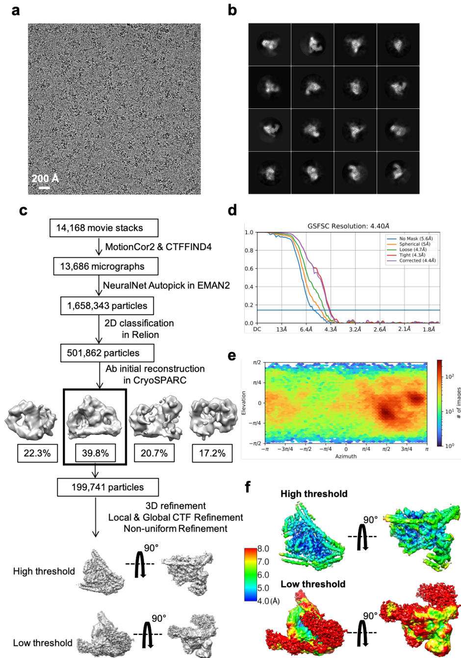
Supplementary information, Fig. S7. Single-particle cryo-EM analysis of the MACOM/MAC complex. a Representative motion-corrected cryo-EM micrograph. b Reference-free 2D class averages. c Workflow of the data processing. d Gold standard FSC plots calculated in cryoSPARC. e Euler angle distribution of the particle images. f Resolution map for the final 3D reconstruction at high and low threshold levels.
