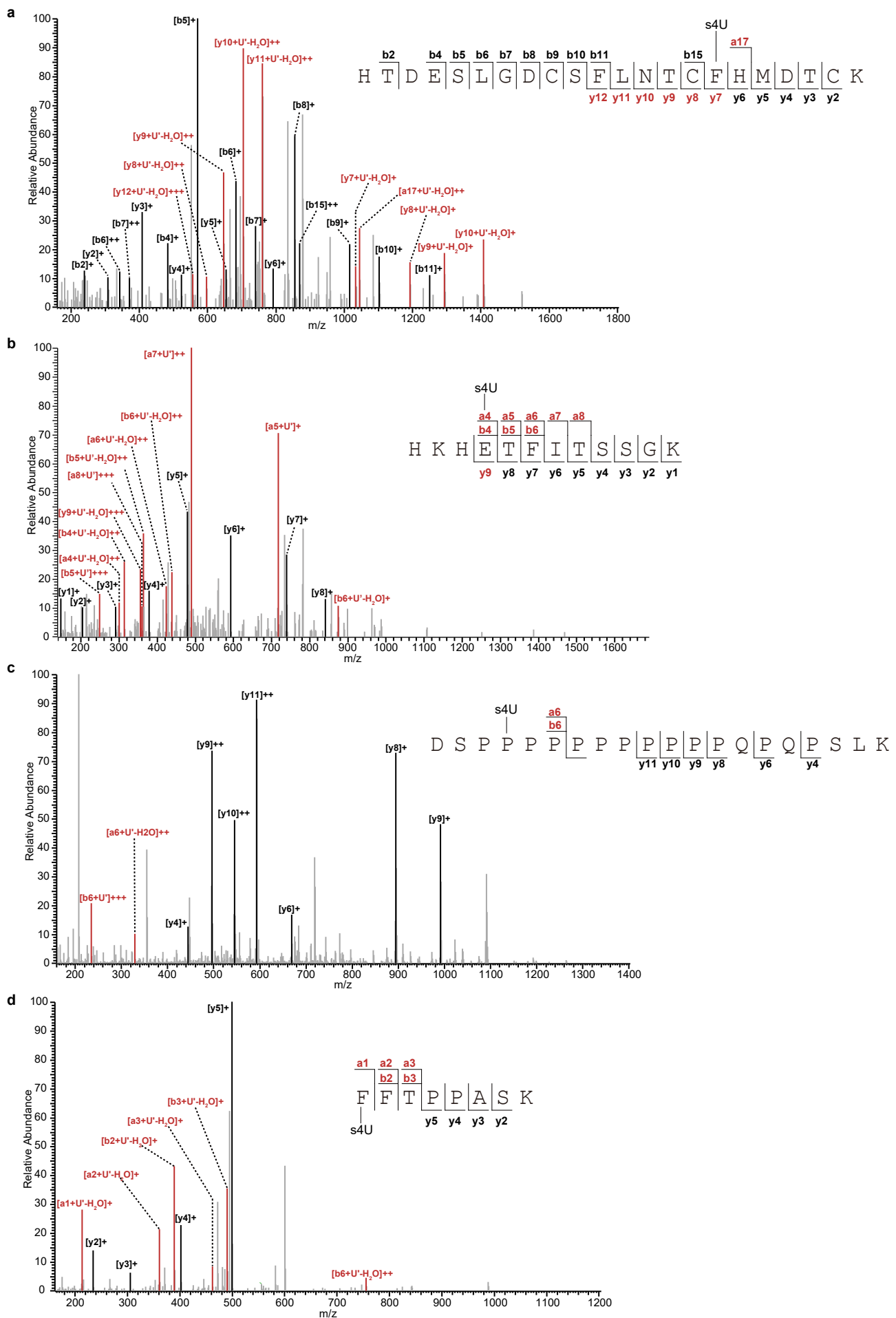
Supplementary information, Fig. S8. MS2 spectrum of a peptide-RNA mononucleotide (s4U minus H2S) crosslink derived from MAC/MACOM, corresponding to Fig. 7a. Raw data were search against a FASTA database consisting of the protein sequences of the proteins in the complexes using RNPxl node combined in PD software with 0.01 FDR.
