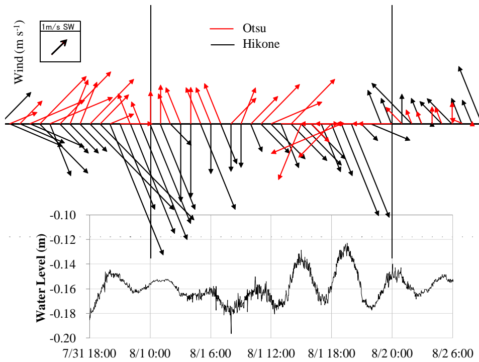
Fig. A1. Time series of the wind vectors measured at the Otsu Meteorological station (top panel) and water level changes at the Yanagasaki pier in the southern basin (bottom panel). The vertical lines indicate midnight on 1 and 2 August 2011.
