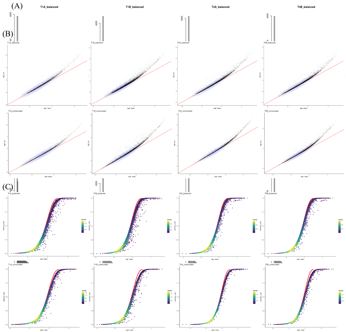
Supplementary Figure 1. Feature-level metrics for balanced and confounded (before correction) study. (A) histograms of mean expression, (B) mean-variance relationship, (C) mean-detection rate relationship
